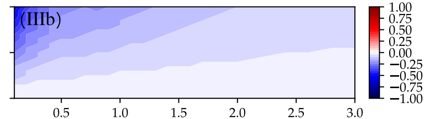
LUT: continental polluted - True: continental clean
