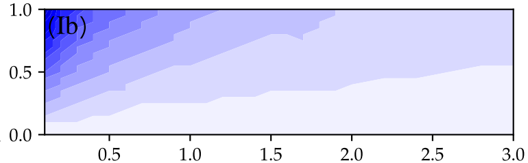
LUT: continental polluted - True: continental clean
