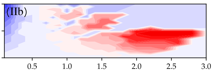
LUT: continental polluted - True: continental clean
