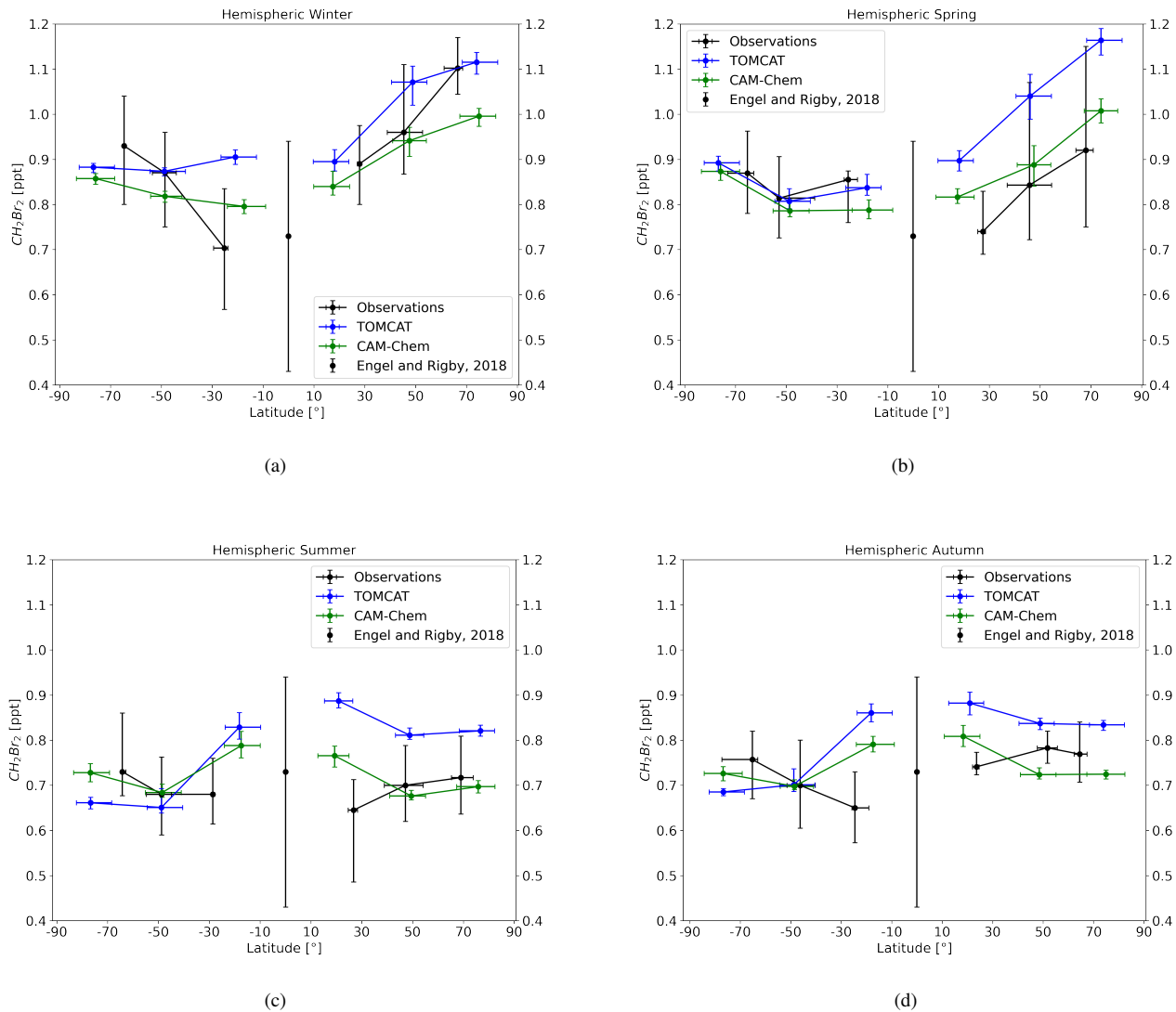
Figure S1. Latitude cross section of tropopause representative mixing ratios of \text{CH}_2\text{Br}_2 using all observation (black) and model results (blue for TOMCAT and green for CAM-Chem) for both hemispheres in (a) winter, (b) spring, (c) summer, and (d) autumn. Data are binned into three latitude bins for each hemisphere: high latitudes (90°–60°), mid latitudes (60°–30°), and low latitudes (30°–0°) and only for data within the 10 K below the dynamical tropopause. Latitudinal position of observational and model bins may differ due to different spatial data coverage of observations and models. Also included are the reference mixing ratios for the tropical tropopause (Engel and Rigby, 2018)
