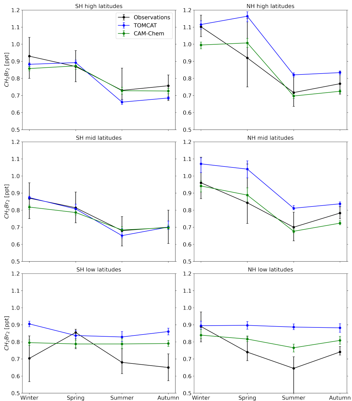
Figure S3. Seasonal cycle of CH 2 Br 2 for the three latitudinal bands: high latitudes (90°–60°), mid latitudes (60°–30°), and low latitudes (30°–0°) and only for data within the 10 K below the dynamical tropopause. Observations are presented in black and model results of TOMCAT and CAM-Chem in blue and green, respectively.
