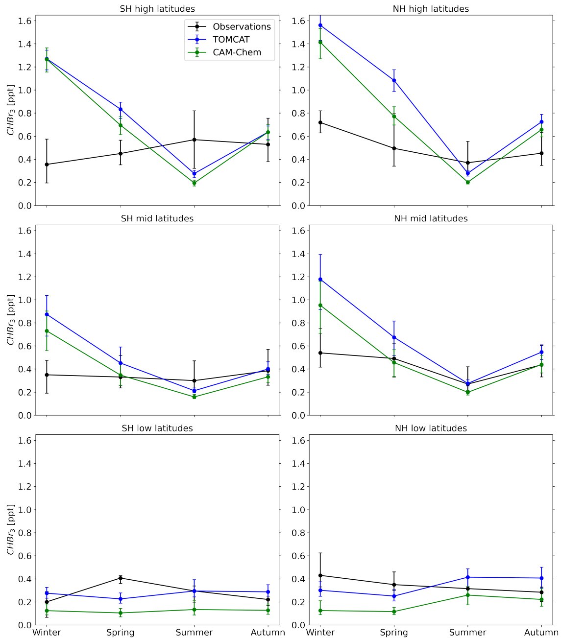
Figure S4. As in Figure S3, but for \text{CHBr}_3 .
