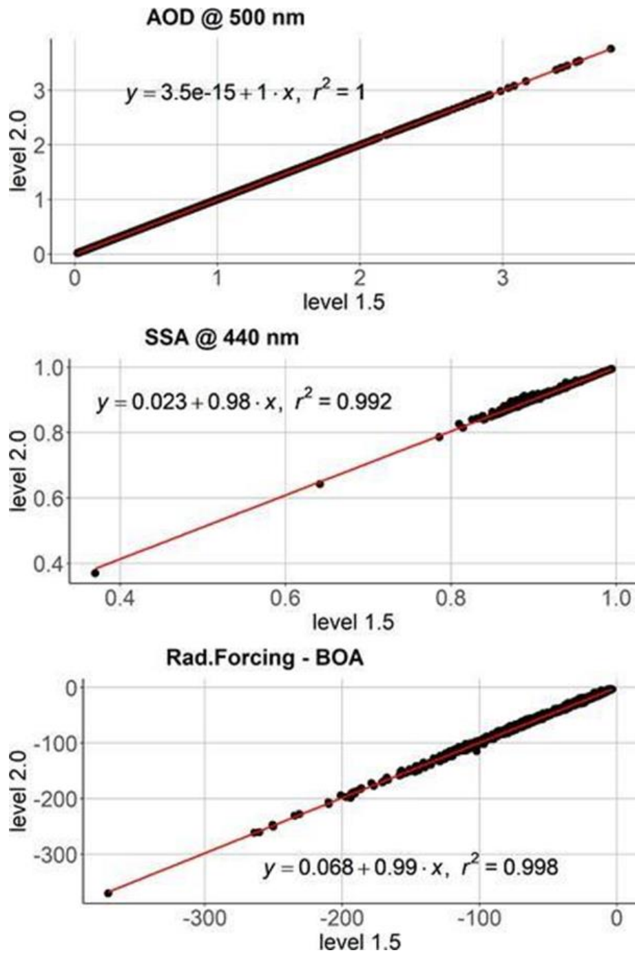
Figure S1: Scatterplot of level 2.0 versus level 1.5 for AOD at 500 nm, SSA at 440 nm and radiative forcing at the surface from AERONET. Red line indicates the best line fit and the coefficients of the linear regression are also presented.
