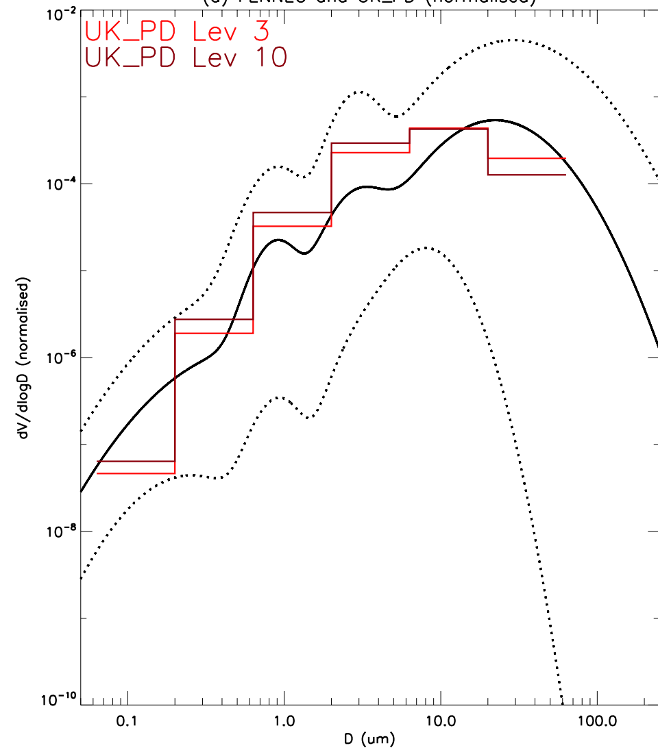
(a) FENNEC and UK_PD (normalised)
