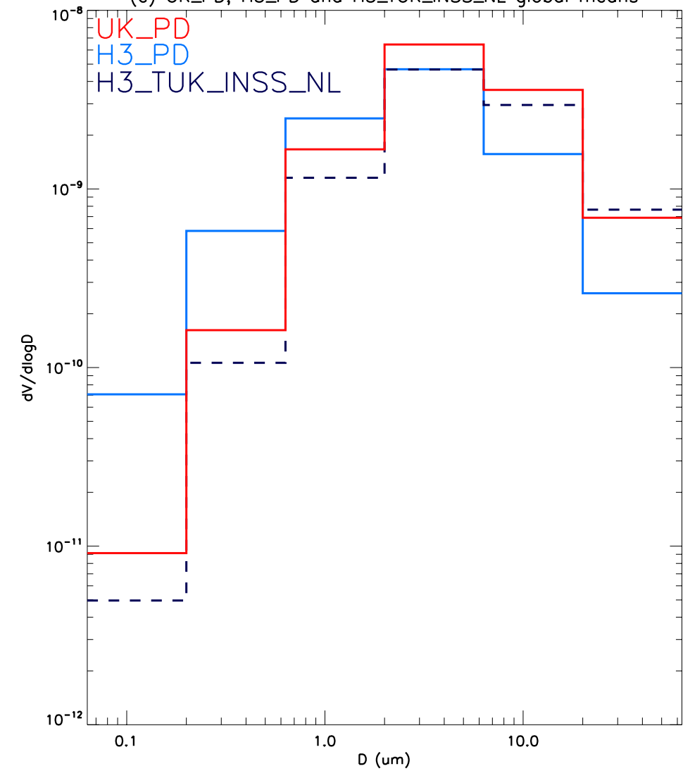
(c) UK_PD, H3_PD and H3_TUK_INSS_NL global means
