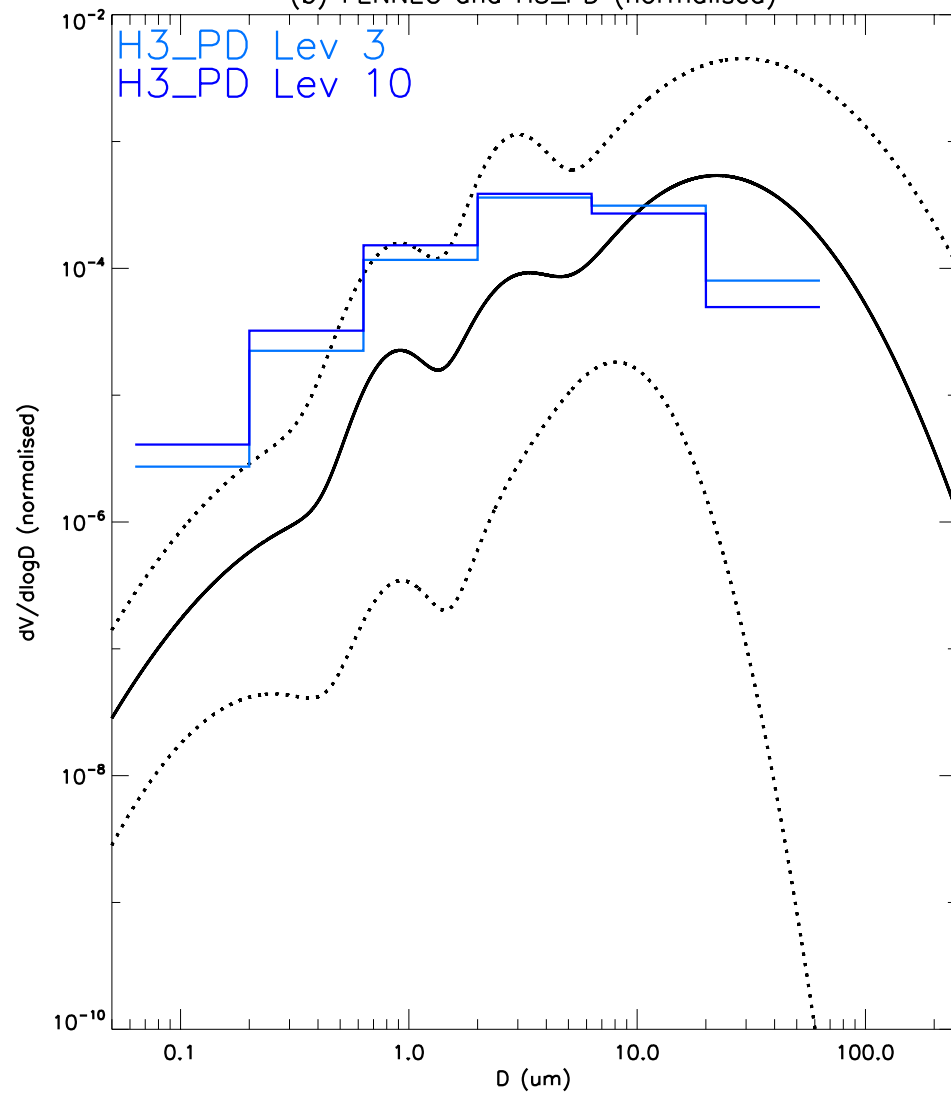
(b) FENNEC and H3_PD (normalised)
