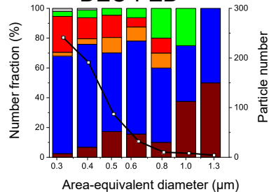
(h) DEC-FEB
