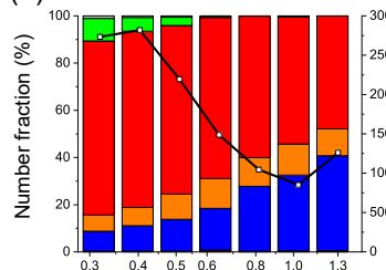
(a) MAR-MAY
