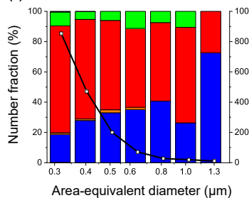
(f) JUN-AUG
