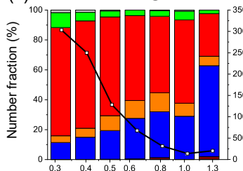
(c) SEP-NOV
