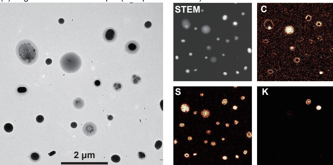
(c) Organic dominant sample (8 September 2017)
