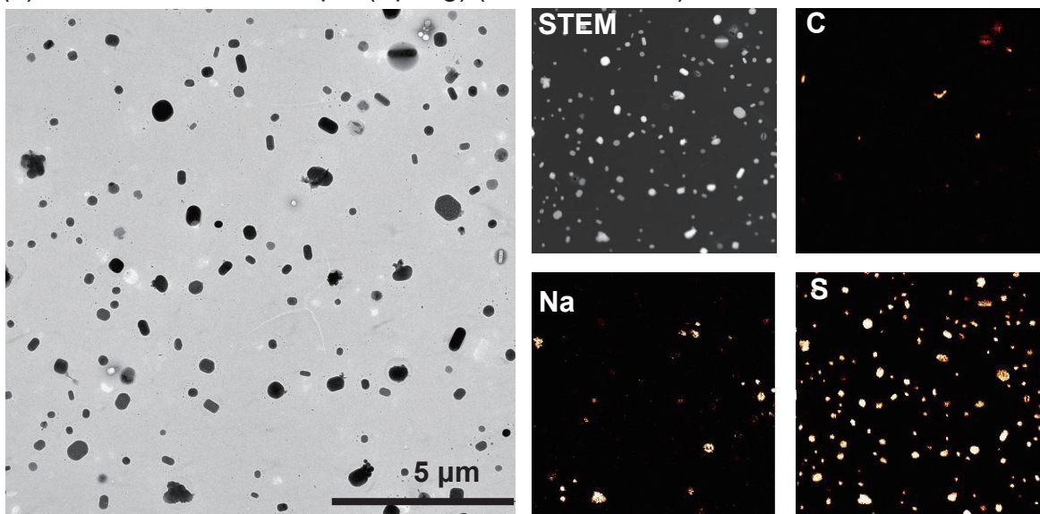
(b) Sulfate dominant sample (Summer) (10 August 2018)
