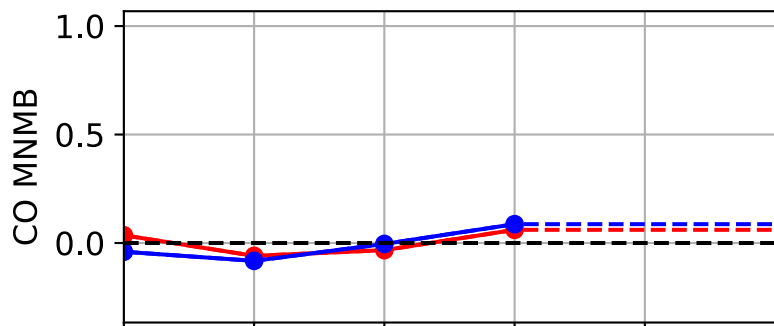
(d1) West Africa [1000-850 hPa]
