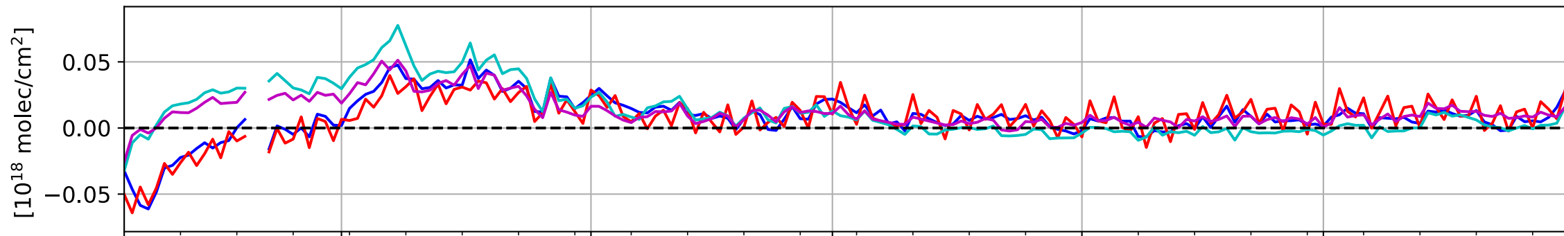
(c) IASI-C
