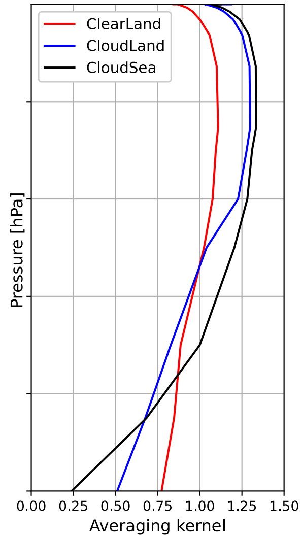
(c) SH
