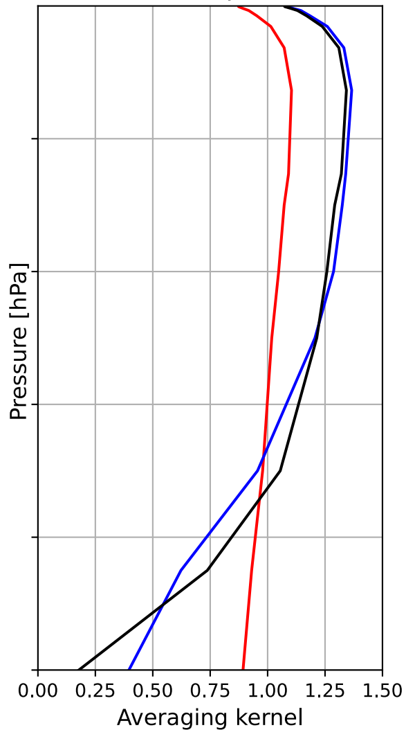
(b) Tropics
