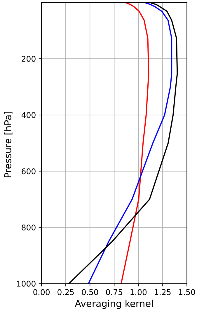
(a) NH
