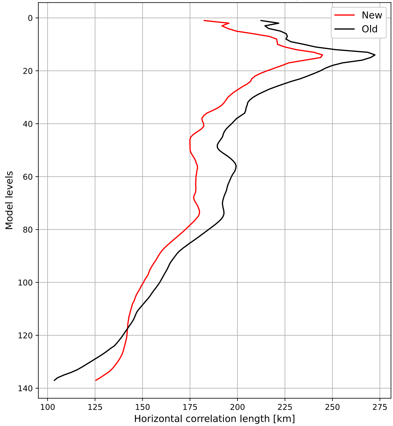
(b) Global mean horizontal correlation profile CO
