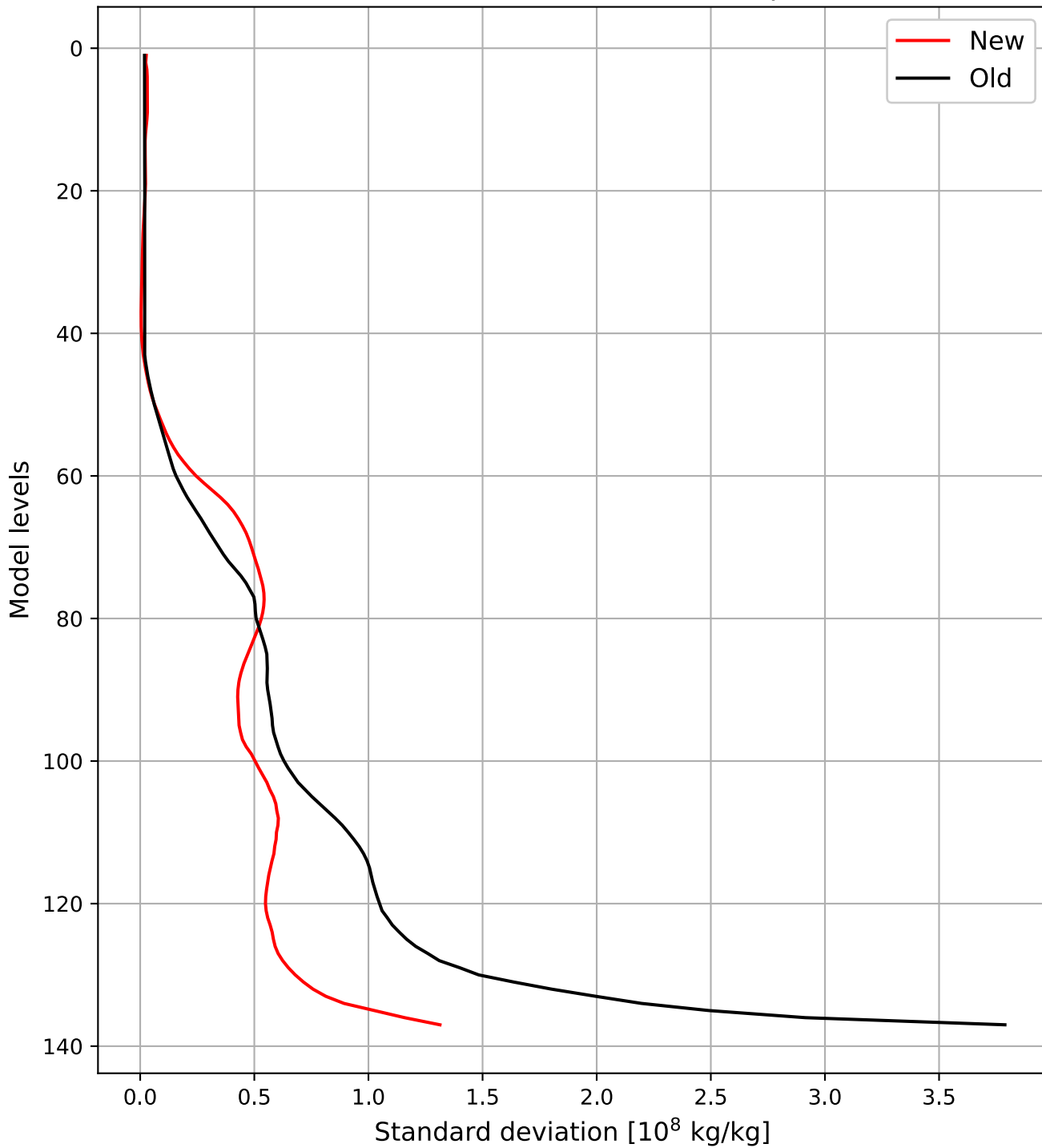
(a) Global mean standard deviation profile CO
