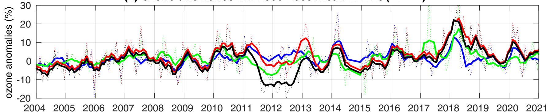
(c) ozone anomalies wrt 2000-2008 mean in DL8 (40 km)
