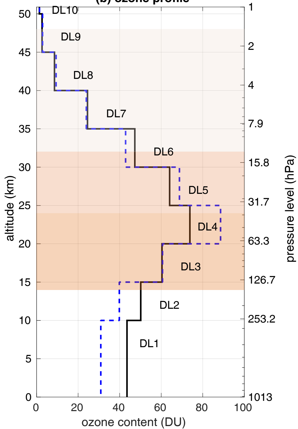
(b) ozone profile
