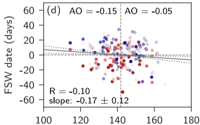
WACCM, CLIM-3D
