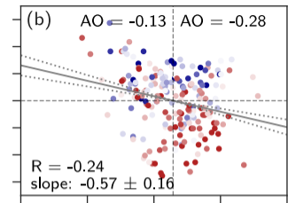
SOCOL-MPIOM, CLIM-3D
