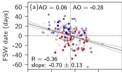
WACCM, CLIM-3D
