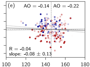
SOCOL-MPIOM, CLIM-3D
