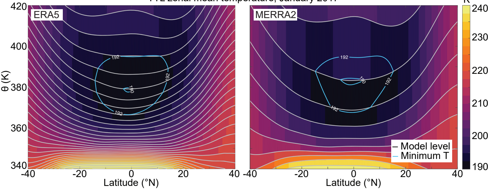
TTL zonal mean temperature, January 2017
