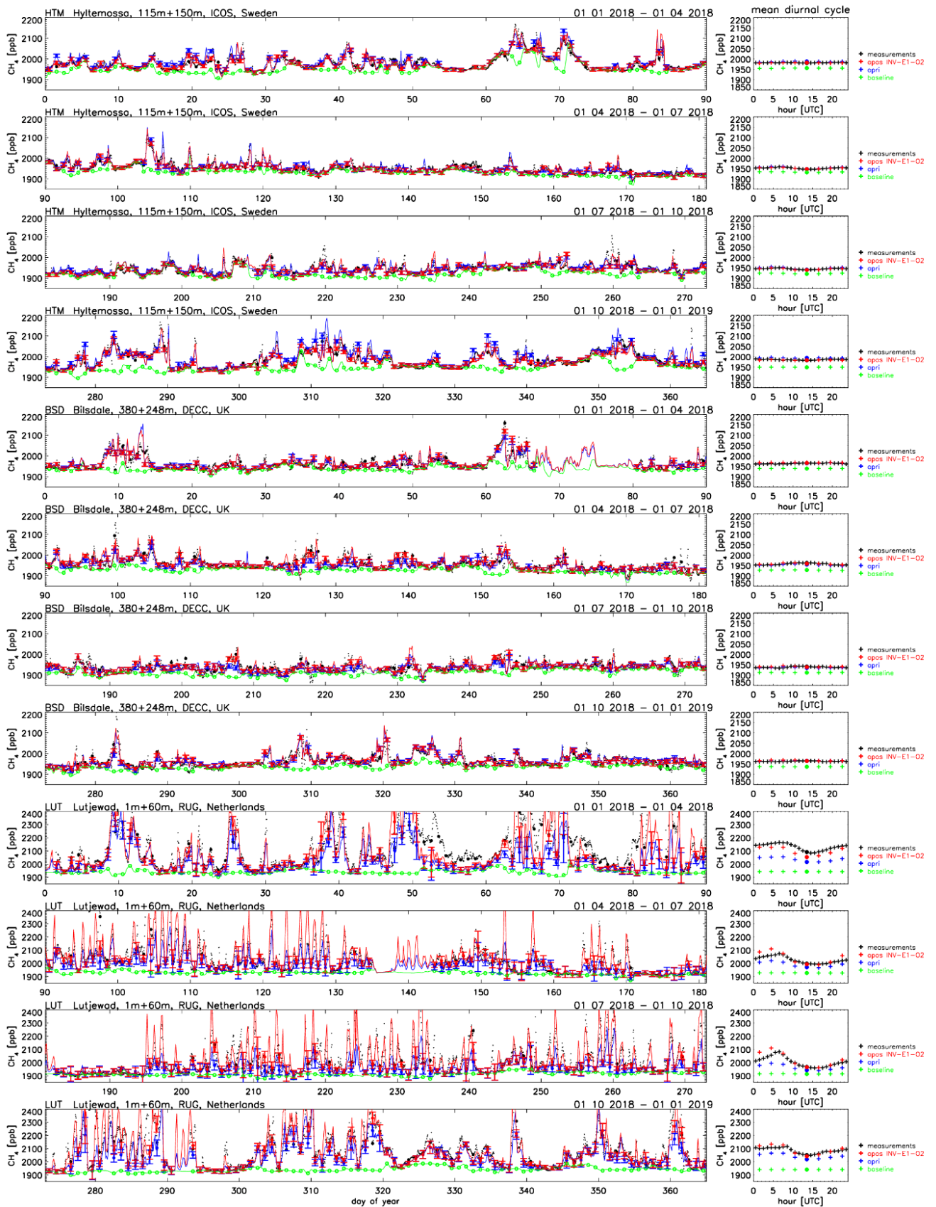
Figure S7: Simulated and observed CH 4 mole fractions at monitoring stations (inversion INV-E1-O2). The main panels (left) show the time series for 3-months periods. Green curves show the baselines, blue the prior simulations, and red the posterior simulations. Small black dots: Hourly-averaged observations. Solid black circles: assimilated observations. Colored circles show the corresponding assimilated values and error bars the applied model representation error. The smaller figures on the right side show the average diurnal cycle for each 3-months period.
