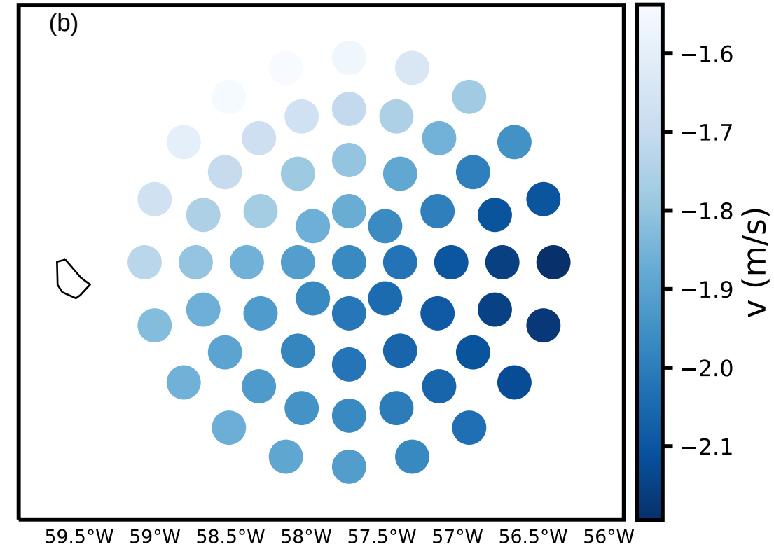
v at 500 m
