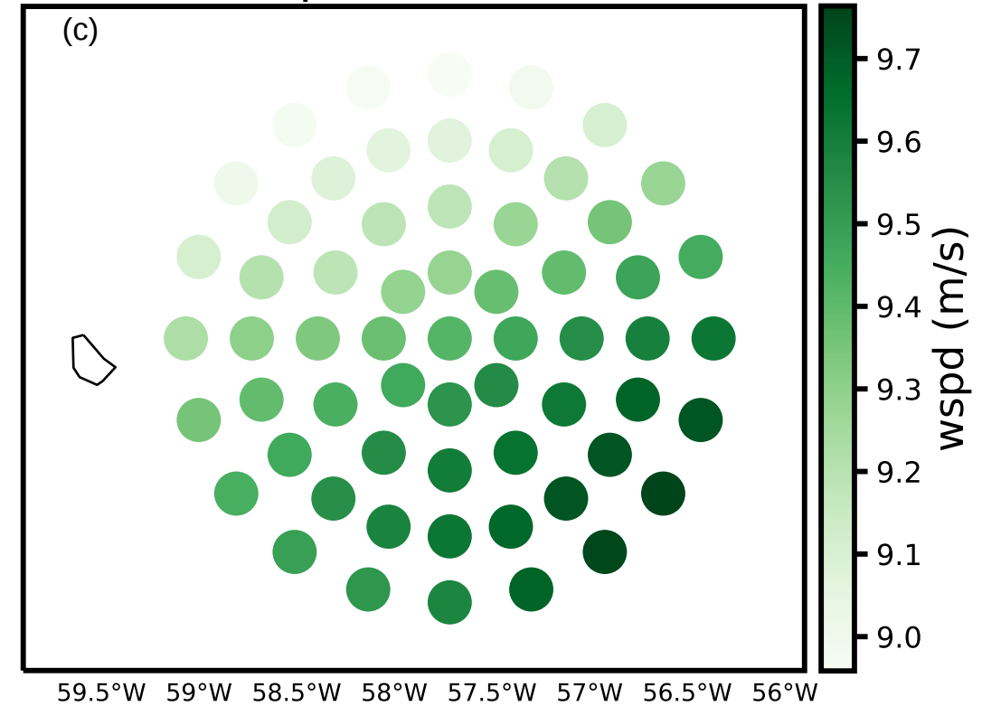
wspd at 500 m
