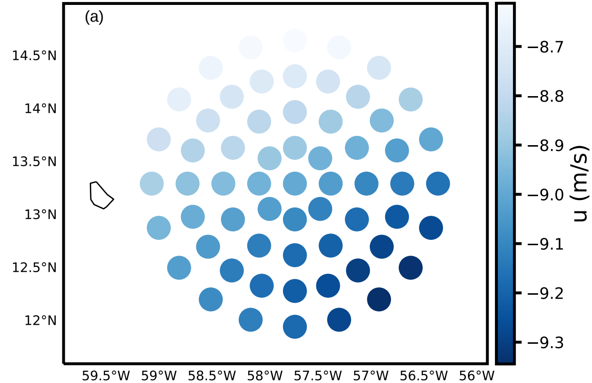
u at 500 m
