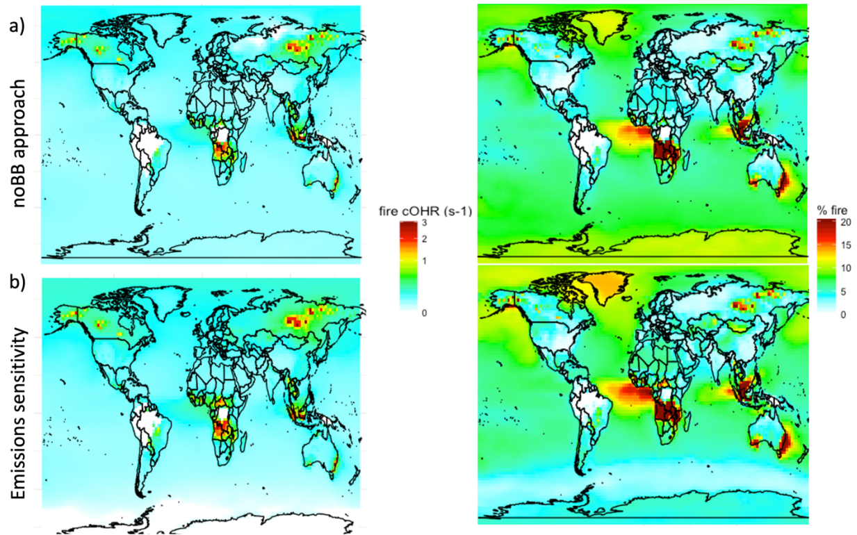
Fig S3: Annual 2019 mean surface OHR and percent OHR attributed to fires using two approaches a) subtracting out no fire simulation versus b) emissions sensitivity runs of 1.05 and 0.95 times fire emissions scaled up to equal an 100% perturbation
