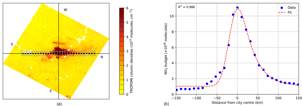
Figure 3. Estimation of the NO 2 lifetime from a pattern above Riyadh on 11 March 2020: (a) NO 2 plume rotated with its wind direction around the source (star) to an upwind–downwind pattern. Grey boxes centred around black points indicate the extent of the spatial integration of NO 2 columns to obtain the NO 2 line density. Values of cardinal points are noted in black. (b) Corresponding line densities (points) representing the downwind evolution of NO 2 as a function of the distance to Riyadh’s city centre and the corresponding fit according to the exponentially modified Gaussian function (dashed line).
