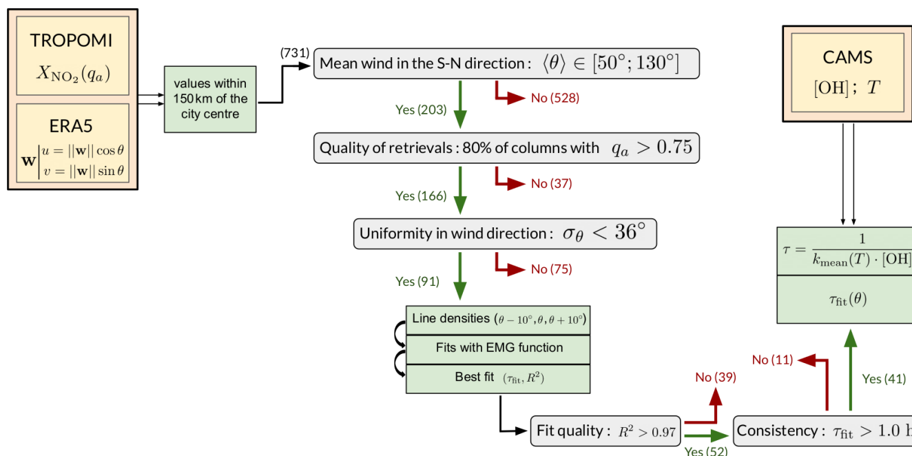
Figure 4. Selection method for NO 2 patterns over Riyadh. Datasets (yellow-orange) are used to calculate the quantities (light green) that are submitted to different tests (grey). A total of 731 patterns are progressively conserved (green arrows) or rejected (red arrows). At each stage, the number of conserved or rejected patterns are noted within brackets (the value is only given for calculations performed at level \mathcal{B} ). This selection process compares the lifetimes estimated by the EMG function fitting with TROPOMI line density profiles to the lifetimes calculated according to Eq. (2) with CAMS data.
