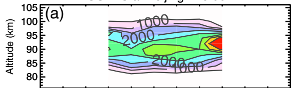
OSIRIS at Beijing ~18:00 LT
