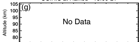
OSIRIS at Haikou ~18:00 LT
