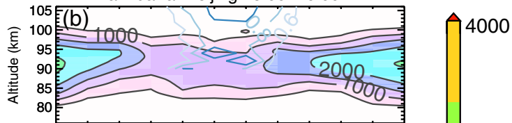
Na Lidar at Beijing 18:00–20:00 LT
