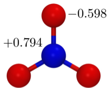
(c) \text{NO}_3^-
