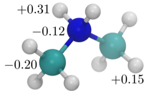
(e) (\text{CH}_3)_2\text{NH}_2^+
