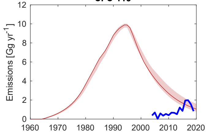
CFC-115
