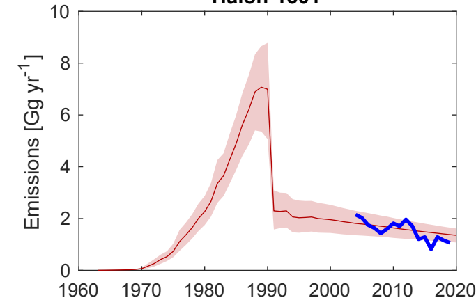
Halon-1301
