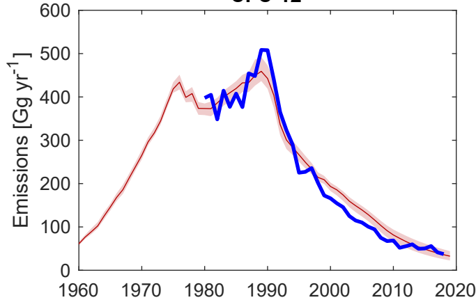
CFC-12
