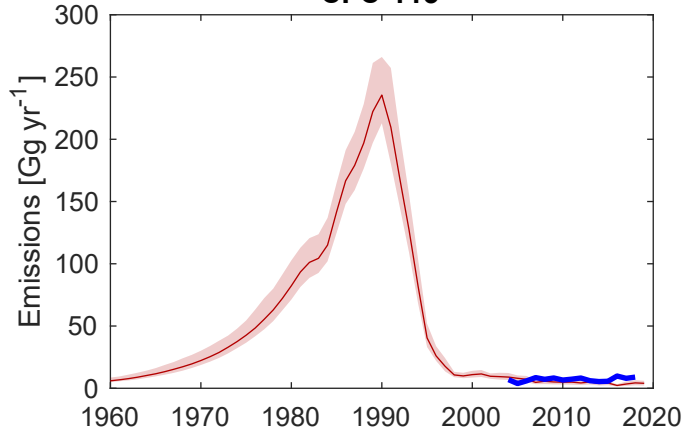
CFC-113
