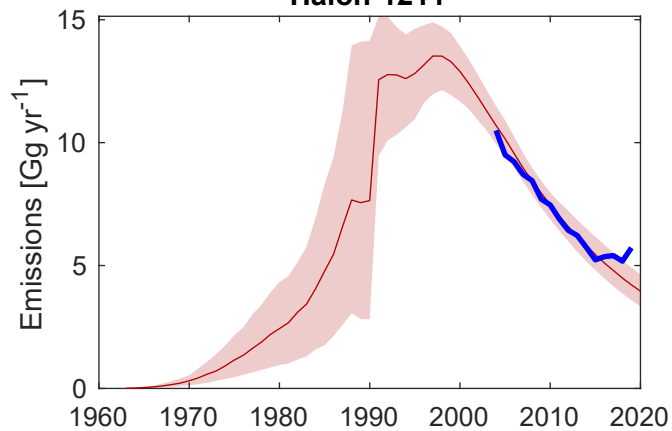
Halon-1211
