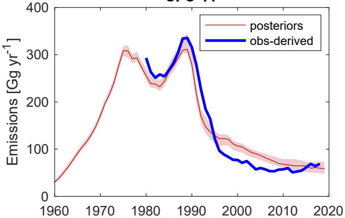
CFC-11
