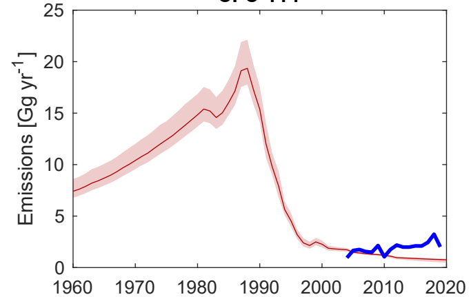
CFC-114
