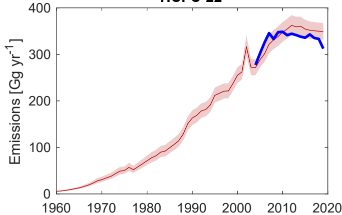
HCFC-22
