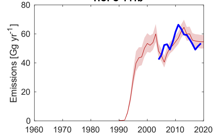
HCFC-141b
