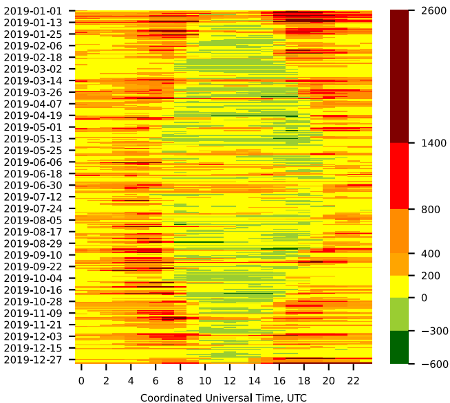
(a) Contrail cirrus net RF ( \text{mW m}^{-2} )
