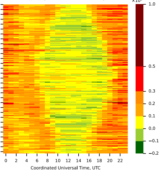
(b) \text{EF}_{\text{contrail}} per contrail distance ( \text{J m}^{-1} )
