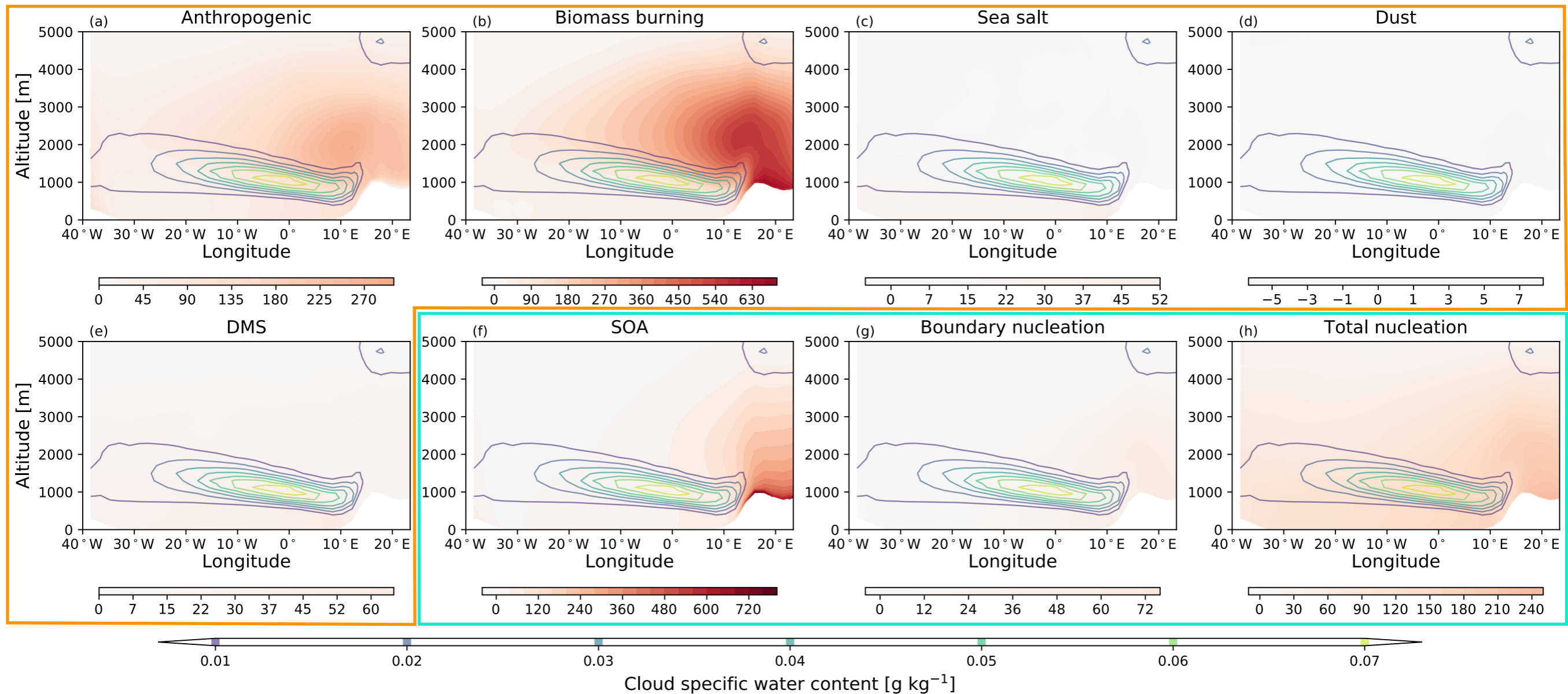
Contribution of different sources to CCN number concentration at 0.2 % supersaturation [ \text{cm}^{-3} ]
