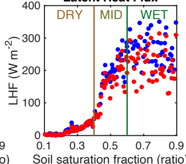
(f) Land-Surface Latent Heat Flux
