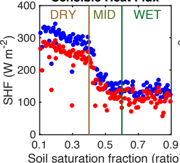
(e) Land-Surface Sensible Heat Flux
