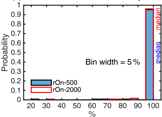
(a) Low Cloud Counts / All Cloudy Counts
