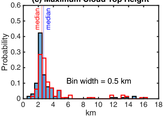
(c) Maximum Cloud Top Height
