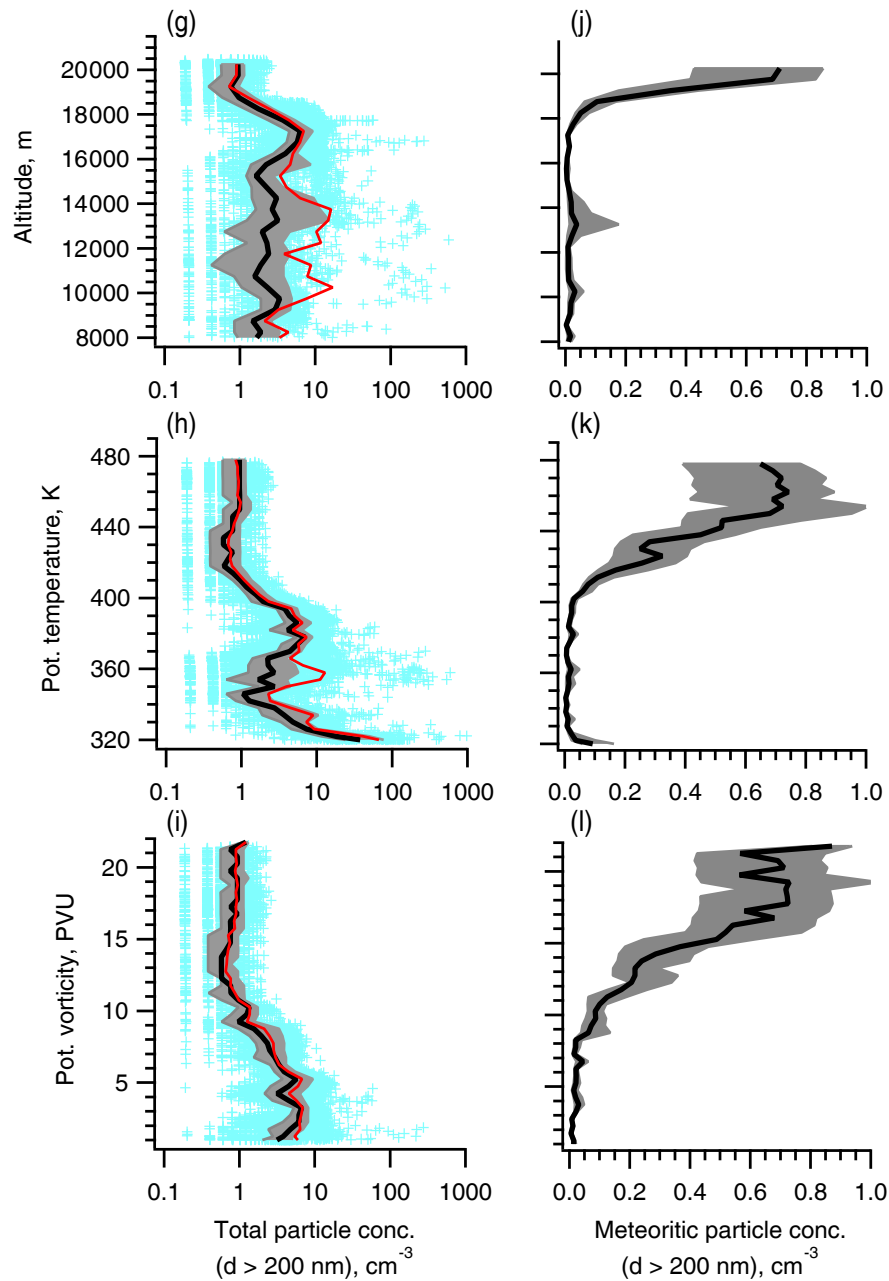
StratoClim 2017
