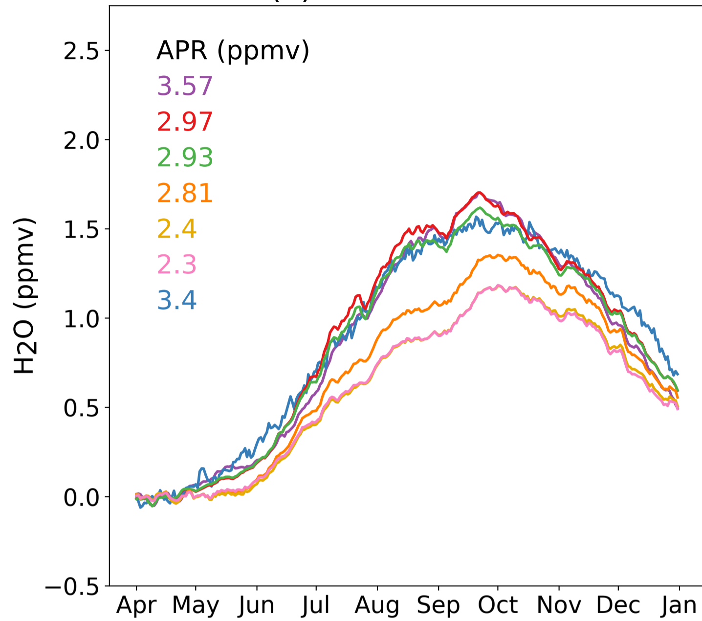
(a) AMA at 80 hPa
