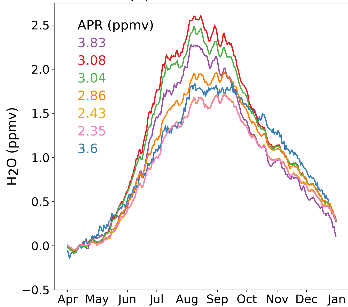
(b) AMA at 100 hPa
