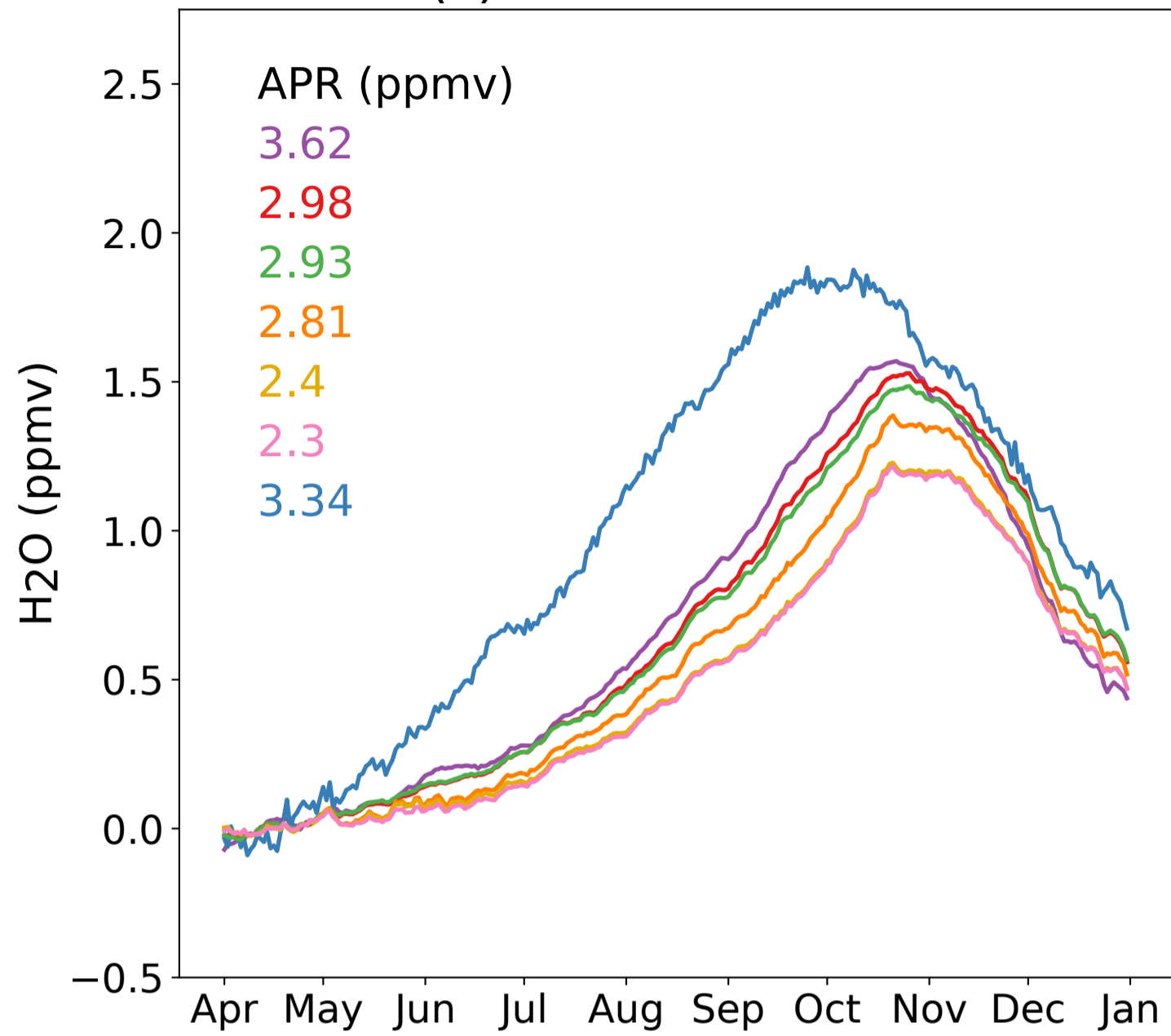
(c) NAMA at 80 hPa
