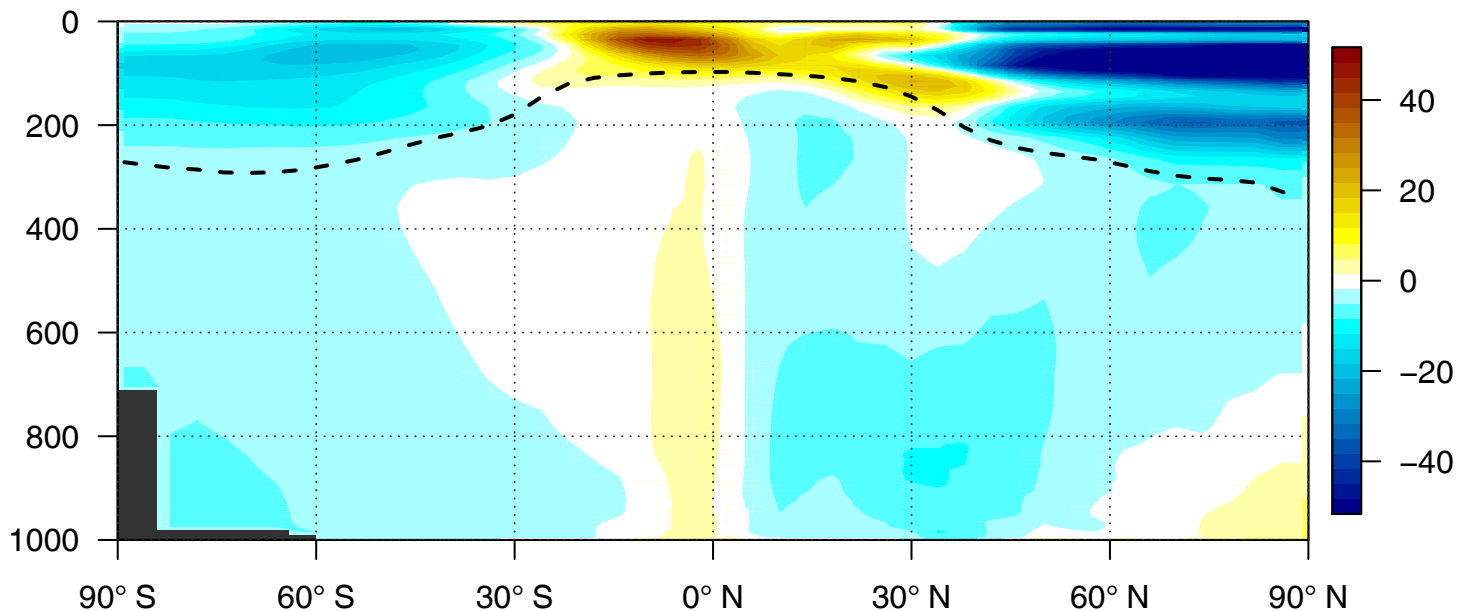
(a) Zonal mean d\text{CH}_4 (WC - A priori) [ppb] 2010/05
