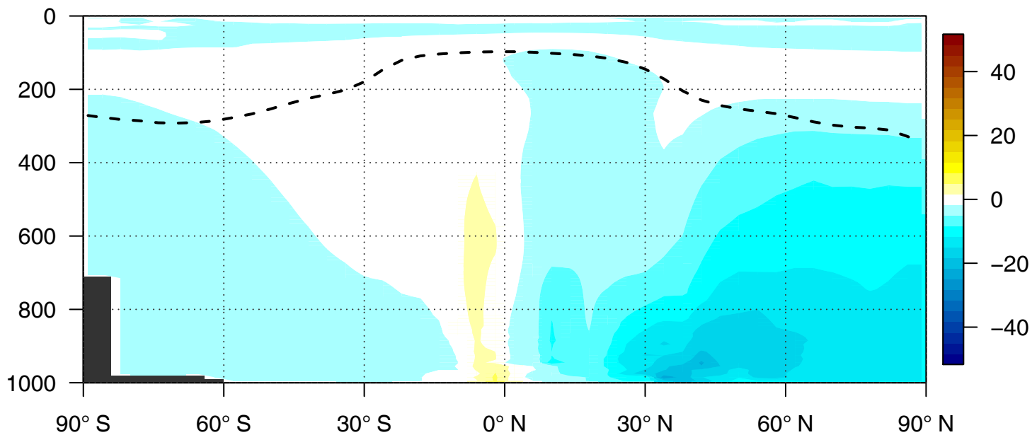
(b) Zonal mean d\text{CH}_4 (SC - A priori) [ppb] 2010/05
