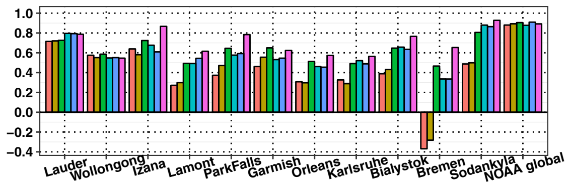
GEOS-Chem vs. TCCON correlation
