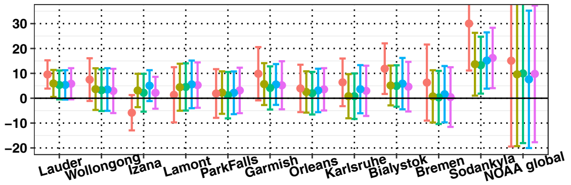
GEOS-Chem vs. TCCON bias and scatter [ppb]
