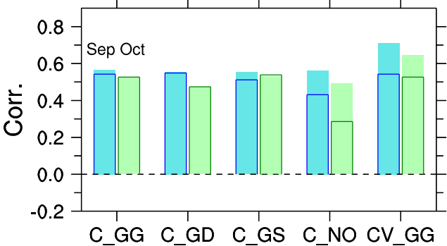
(c) CO 2
