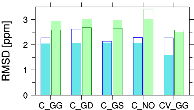
(c) CO 2
