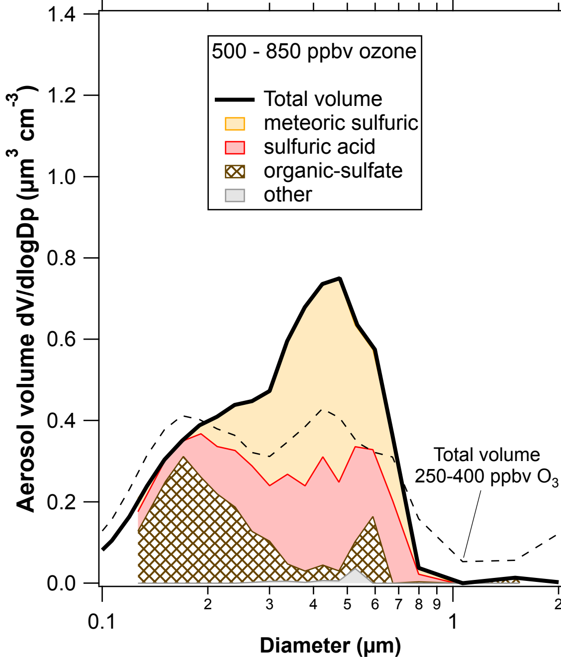
ATom2 January-February 2017
