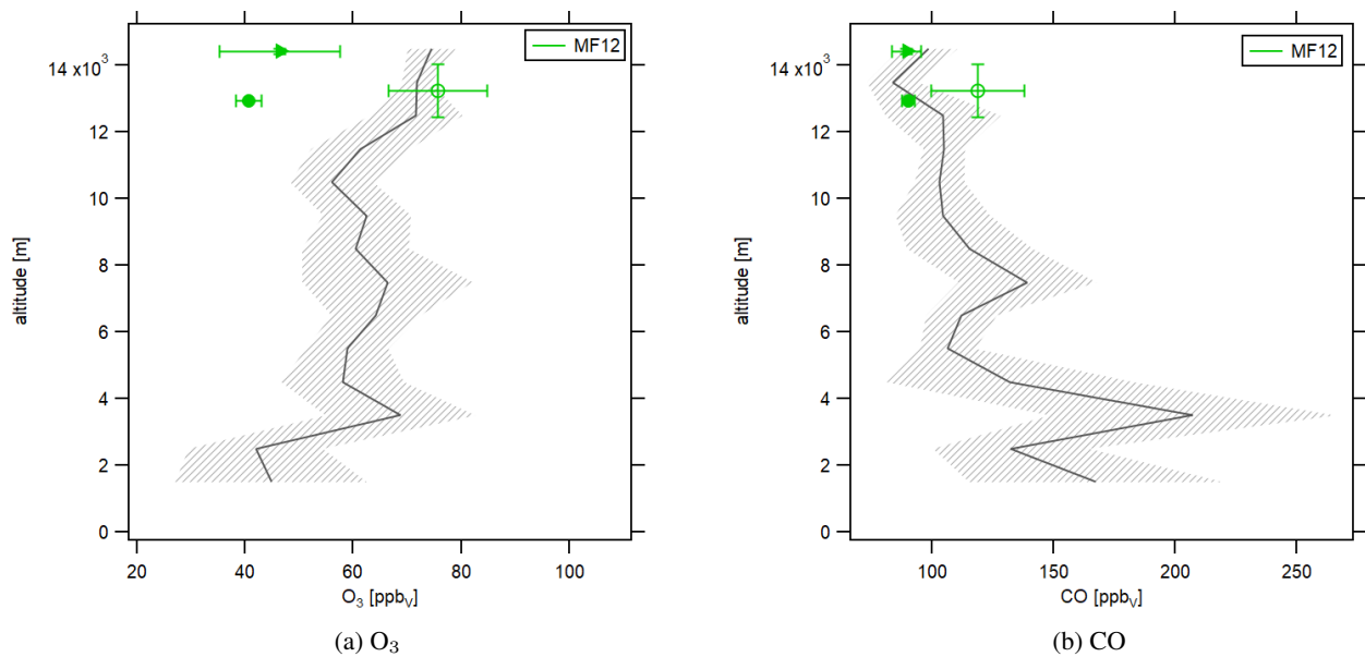
Figure S6. Southern hemisphere ( < 5^\circ N ) background profiles for O_3 and CO including MF12 average concentrations (as shown in Figure 4) for comparison.
