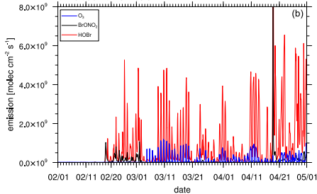
Simulation 3 - emission
