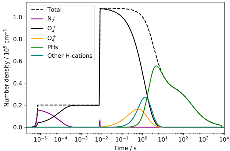
(a) Positive ions (75 km)
