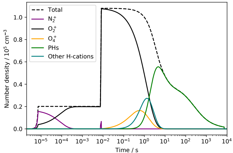
(b) Positive ions (75 km)
