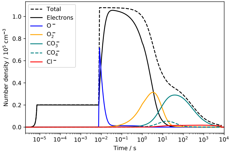
(a) Negative species (75 km)
