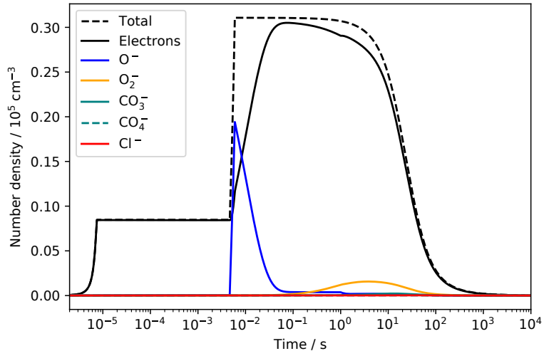
(b) Negative species (80 km)
