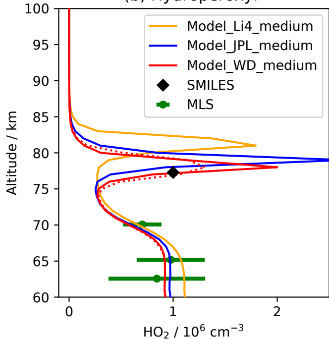
(b) Hydroperoxyl
