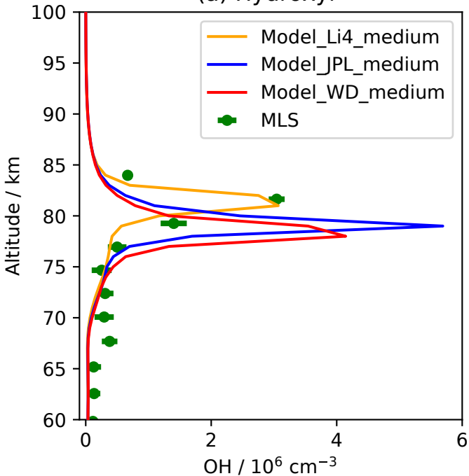
(a) Hydroxyl
