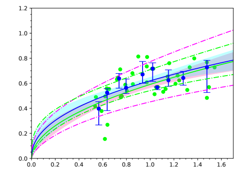
(10) Spatial plates
