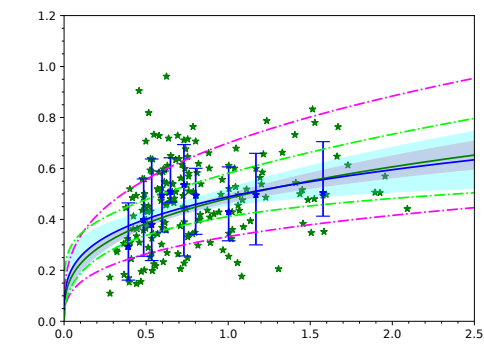
(7) Bullet rosettes
