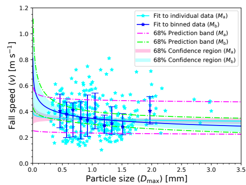
(4) Capped columns
