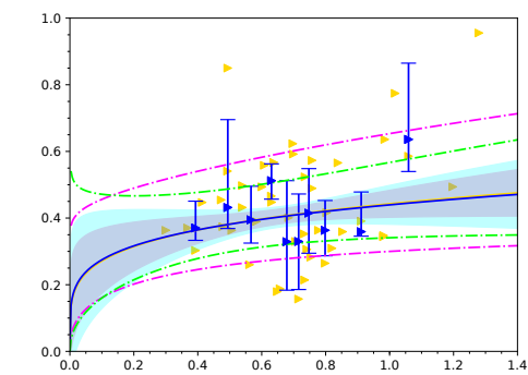
(13) Ice particles
