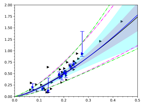
(15) Spherical
