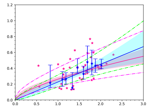
(9) Side planes
