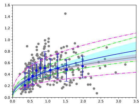
(14) Irregulars
