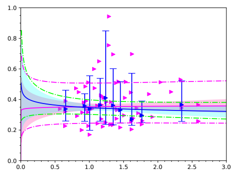
(5) Plates
