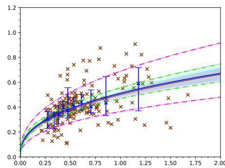
(8) Branches
