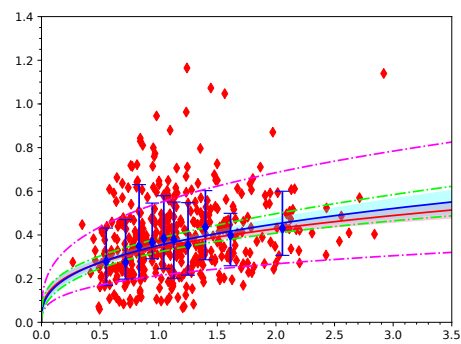
(11) Spatial stellar
