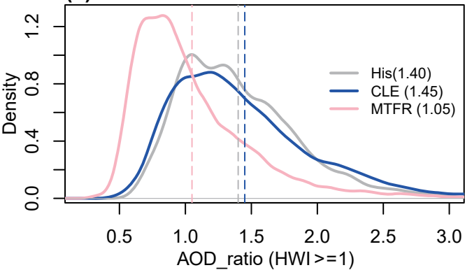
(a) HadGEM3-GC2
