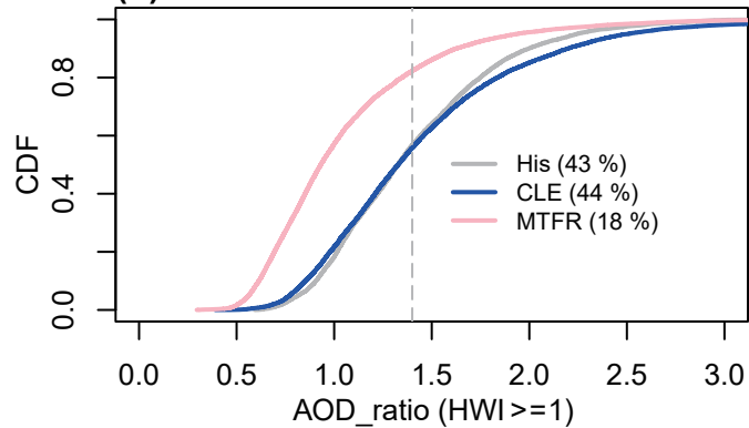
(b) HadGEM3-GC2
