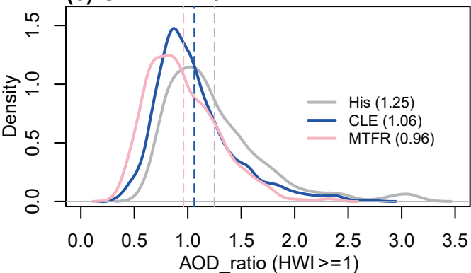
(c) GFDL-CM3
