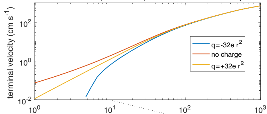
Electric field ( 400 \text{ V cm}^{-1} ) effect on terminal velocity
