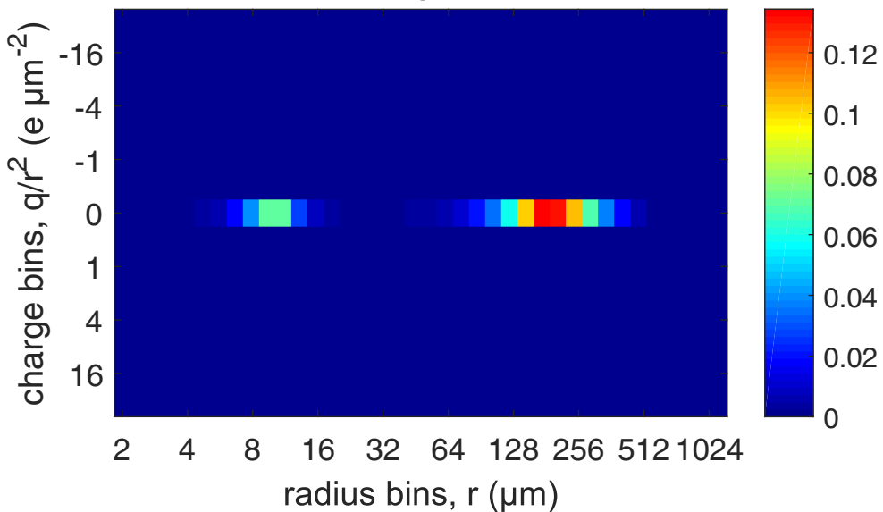
(a) uncharged droplets under no field mass distribution ( \text{g m}^{-3} ) after 60 min
