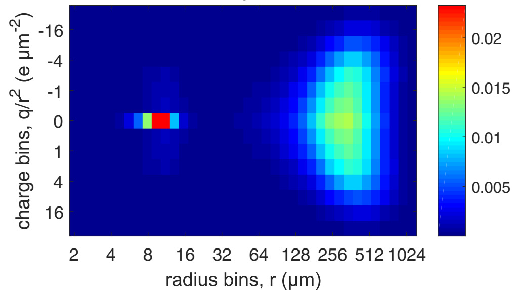
(b) charged droplets under no field mass distribution ( \text{g m}^{-3} ) after 60 min
