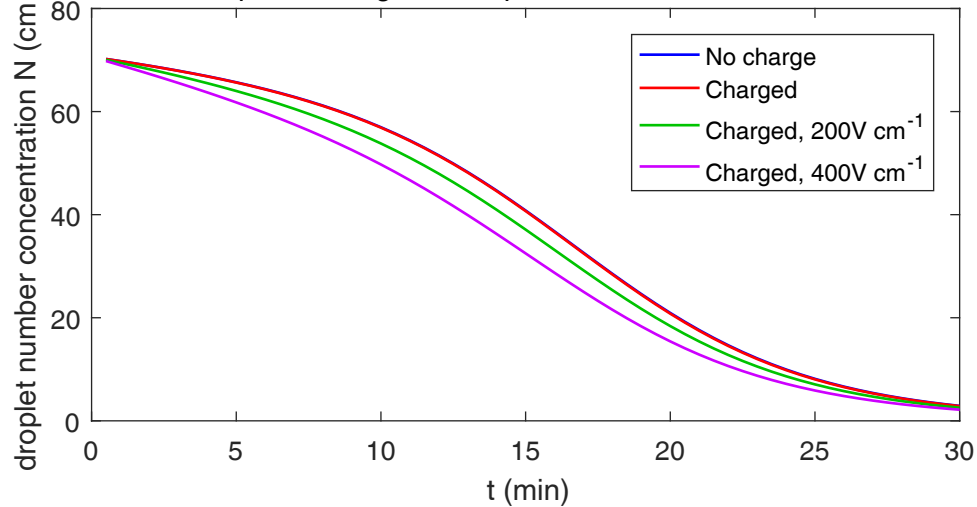
temporal changes in droplet number concentration
