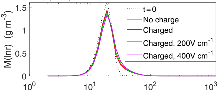
(b) droplet size distribution after 15 min
