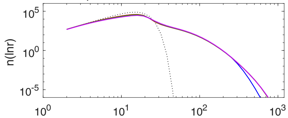
droplet size distribution after 22.5 min
