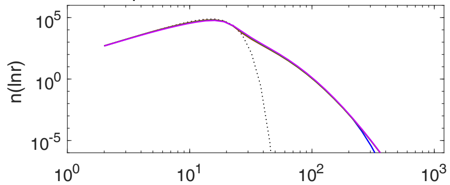
droplet size distribution after 15 min
