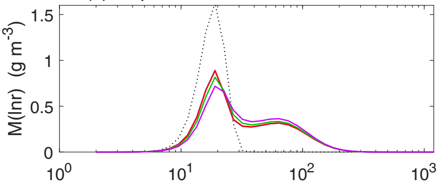
(c) droplet size distribution after 22.5 min
