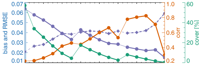
OMAERUV vs. POLDER-SRON
