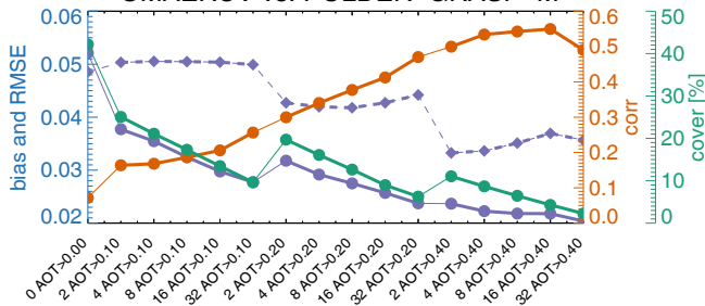
OMAERUV vs. POLDER-GRASP-M
