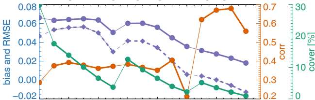
OMAERUV vs. POLDER-GRASP-M
