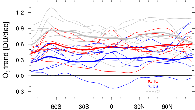
(a) upper stratosphere (1-10 hPa)
