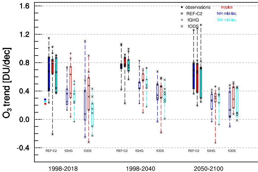
(b) MMM ozone trend, lower stratosphere
