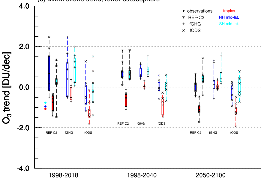
(b) MMM ozone trend, lower stratosphere
