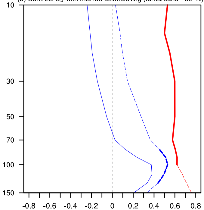
(b) Corr. LS O 3 with mid-lat. downwelling (turnaround - 50° N)
