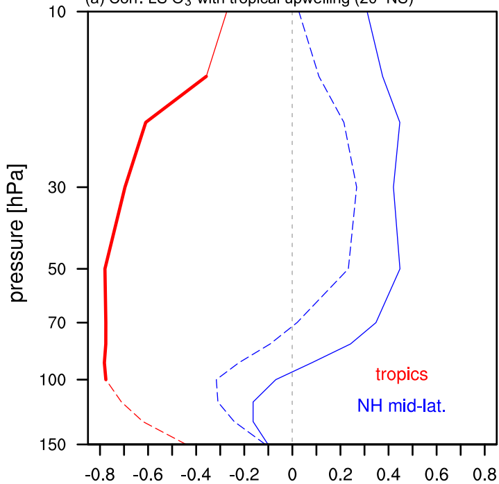
(a) Corr. LS O 3 with tropical upwelling (20° NS)
