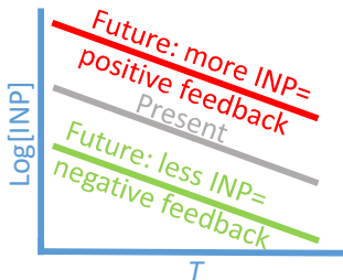
(a) Present day [INP] response (b) [INP] type (slope) response (c) \Delta [INP] response
