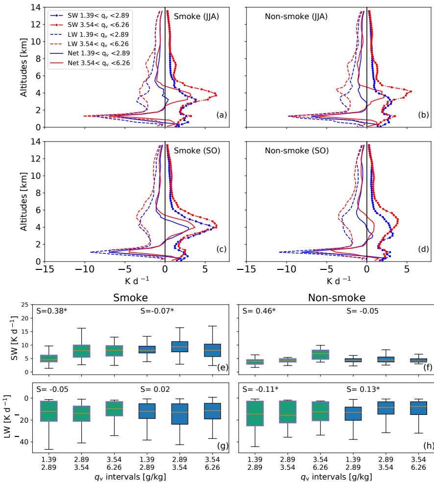
Mean radiative heating profiles q_v intervals
