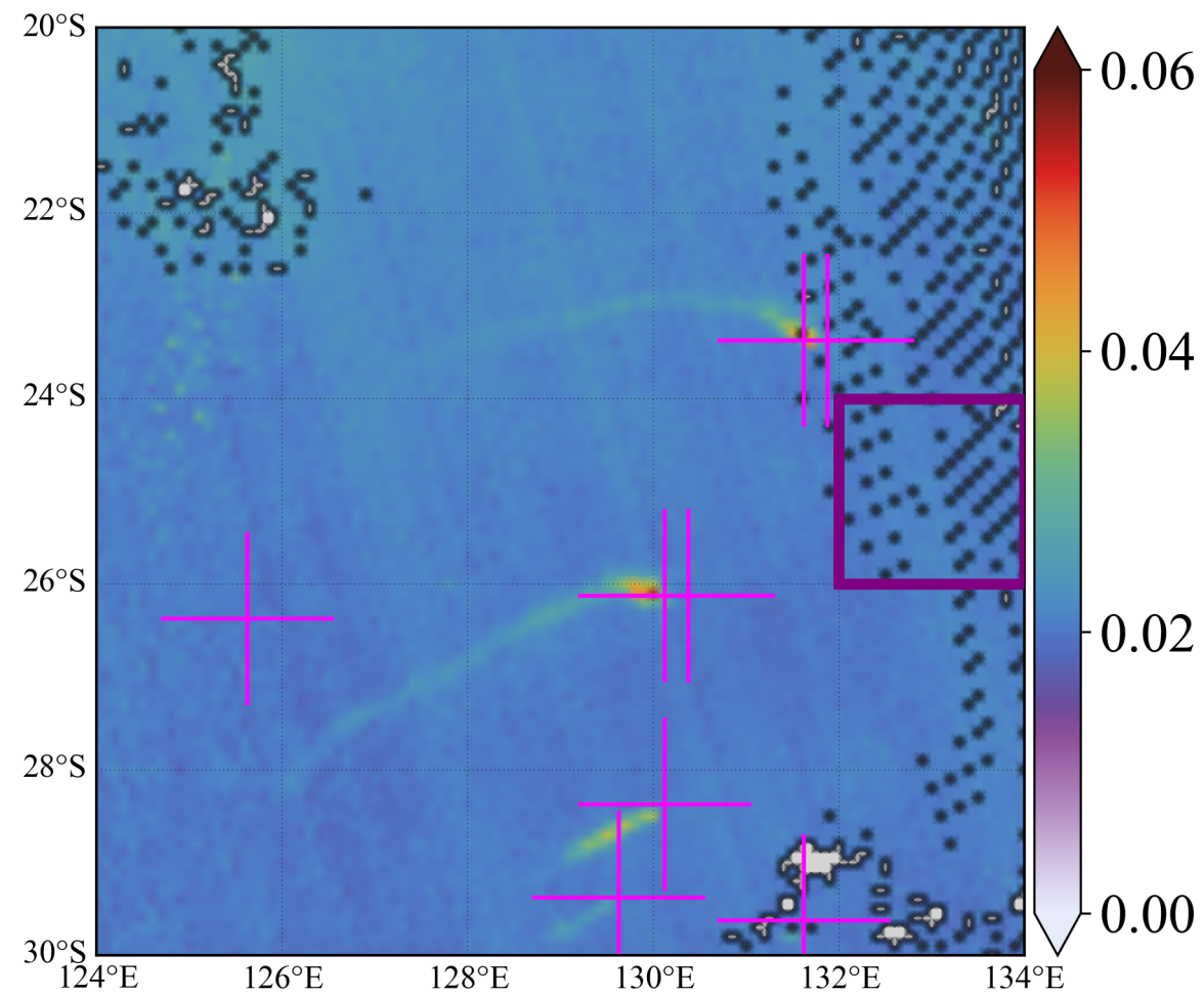
(a) XCO [mol m -2 ] 2018-12-23
