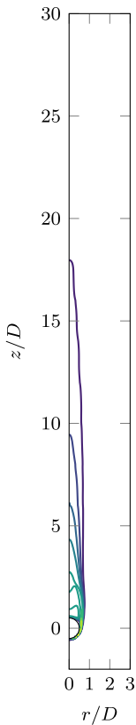
(b) Re = 600
